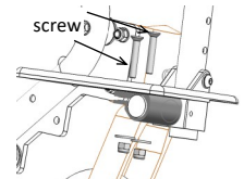
pic. 10.3: Angle Adjustment
