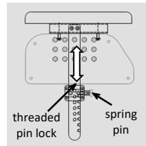
pic. 25: Kit ABS Lateral
