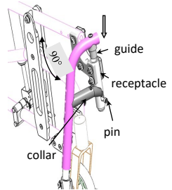
pic. 4: inserting the legrest tube
