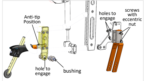
Frame Height Adjustment to 490mm
