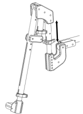
pic. 24: Legrest tube installation/removal
