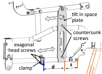
pic. 12.1: Displacement of the seat (folding model)
