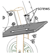
pic. 10.2: Depth Adjustment
