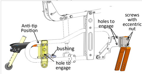
Frame Height Adjustment to 430mm
