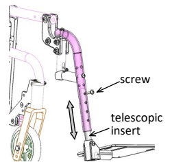
pic. 10.1: Height adjustment
