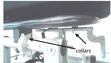
pic. 15: Collars for depth adjustment
