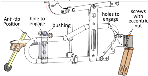
Frame Height Adjustment to 430mm
