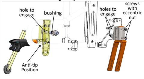
Frame Height Adjustment to 490mm
