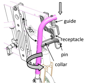
pic. 23: Legrest tube installation/removal
