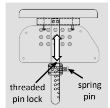
pic. 16: ABS Lateral
